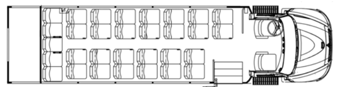
HC350 PLATINUM 31 PASSENGERS + ESCORT, REAR LUGGAGE
