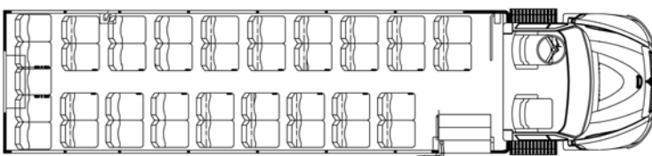
HC380 PLATINUM 39 PASSENGERS + ESCORT
